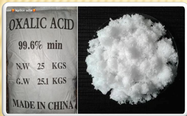
Oxalic Acid
